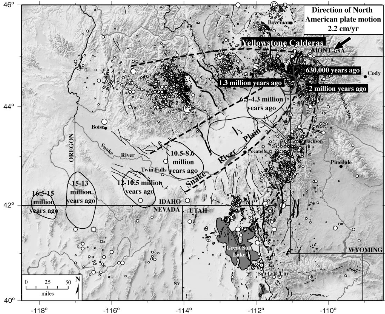
Fig. 1: Volcanic and tectonic features of the Yellowstone-Snake River Plain (YSRP) system. The YSRP study includes southern Idaho, western Wyoming, and southwestern Montana. Y=Yellowstone National Park. Figure after Smith and Siegel (2000), Humphreys et al. (2000), and Christiansen et al. (2002).
