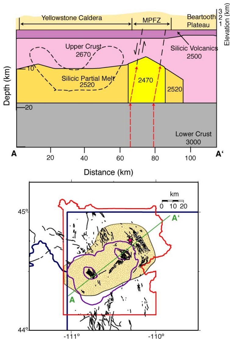
Fig. 8: Cartoon illustrating possible magma movement northeast of the Yellowstone caldera. Southwest dipping extensional faults of the Mirror Plateau Fault Zone (MPFZ) facilitate magma movement. Densities in \text{kg/m}^3 . Red arrows indicate magma movement. Purple outlines the 0.6 Ma caldera. Pink star is the location of Hot Springs Basin Group hydrothermal system. Yellow stipple pattern shows the lateral extent of partial melt derived from our density model.
