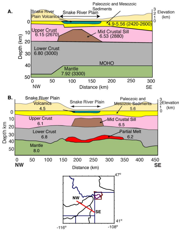
Fig. 4: Crustal structure of the SRP determined from the seismic refraction study of Sparlin et al. (1982): (A) and the seismic receiver function analysis of Peng and Humphreys (1998) (B). Red line on the map represents the approximate location of both profiles. Velocities are in \text{km/s} . Numbers in parentheses are densities in \text{kg/m}^3 . Shaded areas above the models are generalized topography ( \text{km} ).
