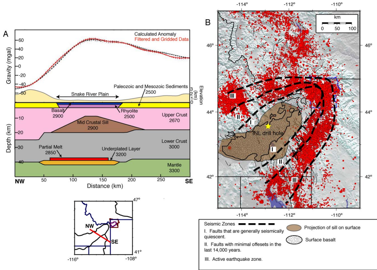
Fig. 5: (A). Cross-section through the YSRP density model (location indicated by the red line on the index map). This location coincides with the area of previous studies of Sparlin et al. (1982) and Peng and Humphreys (1998). All densities in \text{kg/m}^3 . The gravity high south of the SRP is modeled as the continuation of the mid-crustal sill up to 20 km southeast. (B). Map showing the relationship between seismic zones defined by Smith and Braile (1993), seismicity, and the extent of the mid-crustal sill from the density model. Seismicity from a compilation of historic seismicity of the central Intermountain west by Ivan Wong (2006, personal communication) and updated for earthquake catalog data of the Montana Bureau of Mines and Geology, the Yellowstone seismic network (University of Utah Seismograph Stations, UUSS), the Idaho National Laboratory, the Jackson Lake seismic network, U.S. National Seismic Network and the Utah seismic network (UUSS).
