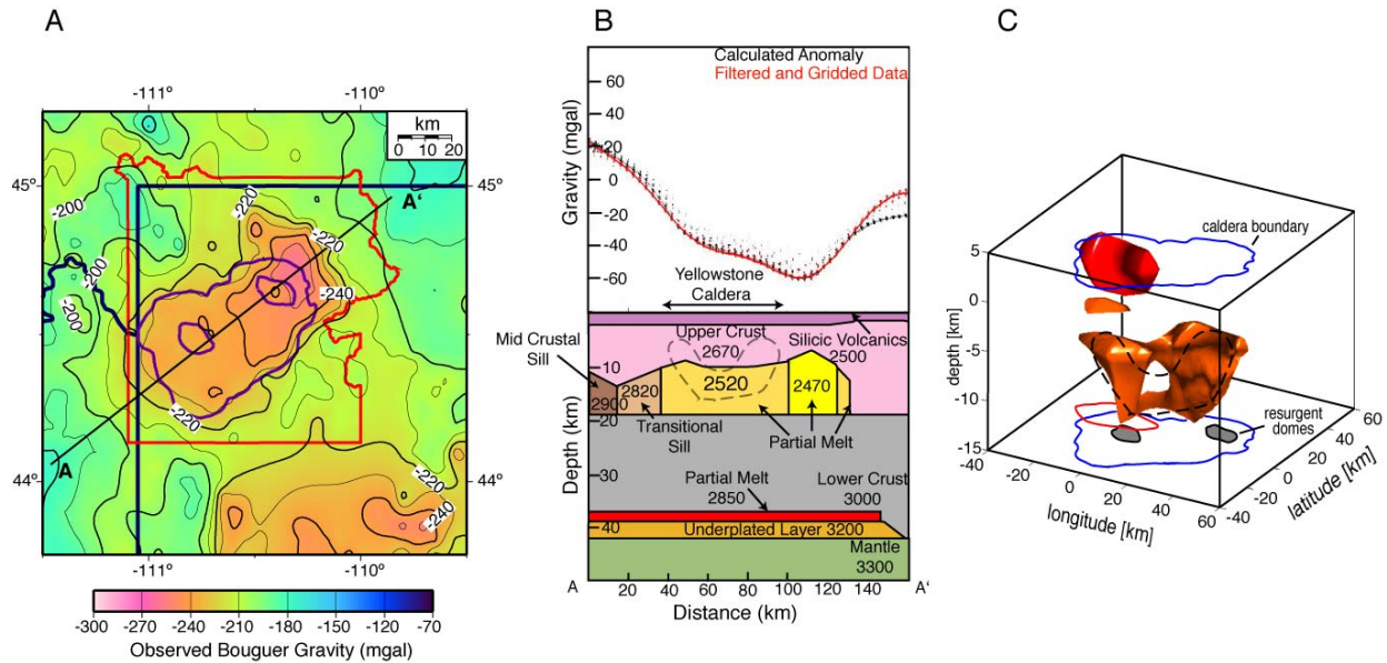
Fig. 7: Gravity profile (A) and cross section through the density model (B) for the Yellowstone area. Densities in \text{kg/m}^3 . The lowest density material extends \sim 20 km beyond the northeastern edge of the caldera. Dashed line represents the approximate location of the seismic low velocity body tomographically imaged by Husen et al. (2004) (C). The steep gravity gradient in this area indicates that the body responsible for the gravity low is closer to the surface here than inside the caldera.
