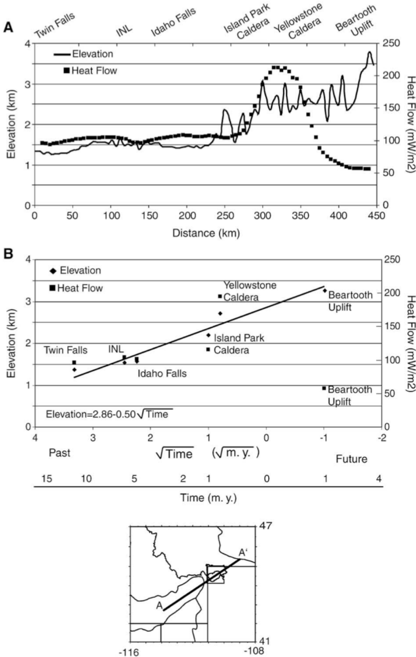
Fig. 13: Generalized relationships between elevation (km), heat flow (mW/m 2 ), and volcanic age along the track of the Yellowstone hotspot. (A). Plots of elevation (km) and surface heat flow from Blackwell and Richards (2004). Heat flow and elevation increase with increasing distance along the hotspot track, with the exception being the undisturbed area east of Yellowstone where the high elevation is due to the Beartooth uplift. (B). A plot of elevation and heat flow vs. the square root of time (where time is the age of silicic volcanic rocks in millions of years from Armstrong et al. (1975)) shows an approximately linear decay of elevation with the square root of time comparable to the lithospheric cooling described by Smith and Braile (1993).
