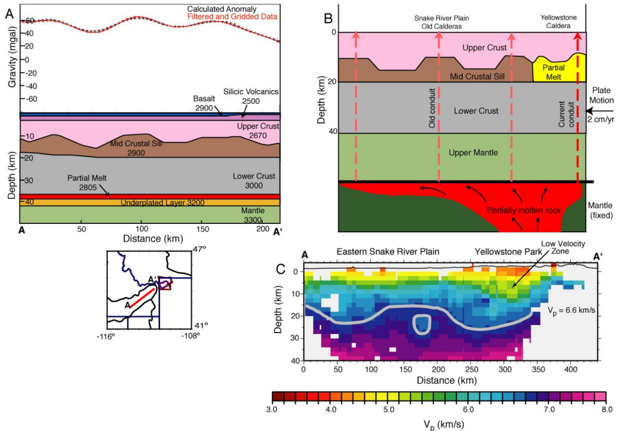
Fig. 6: (A). Cross-section through the density model along the axis of the SRP. A process that could produce the variable thickness observed in the mid-crustal sill is illustrated in (B). As magma rises through the crust it preferentially ascends through volumes that have already been thermally altered, resulting in a thicker sill at these locations. Additional support for this geometry is provided by the seismic tomographic images of Lynch et al. (1997) and Lynch (1998) (C). The V_p = 6.6 km/s contour approximates the top of the mid-crustal sill, and varies in depth along the axis of the SRP.
