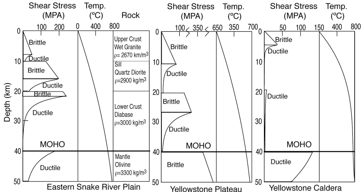
Fig. 11: Strength models of the eastern SRP, Yellowstone Plateau, and Yellowstone caldera. Profile locations and respective strain rates are shown in Figure 10.
