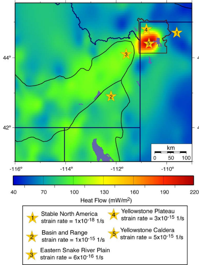
Fig. 10: Map showing the locations of the calculated strength profiles from rheologic modeling. Strain rates at each location from Puskas et al. (2007).
