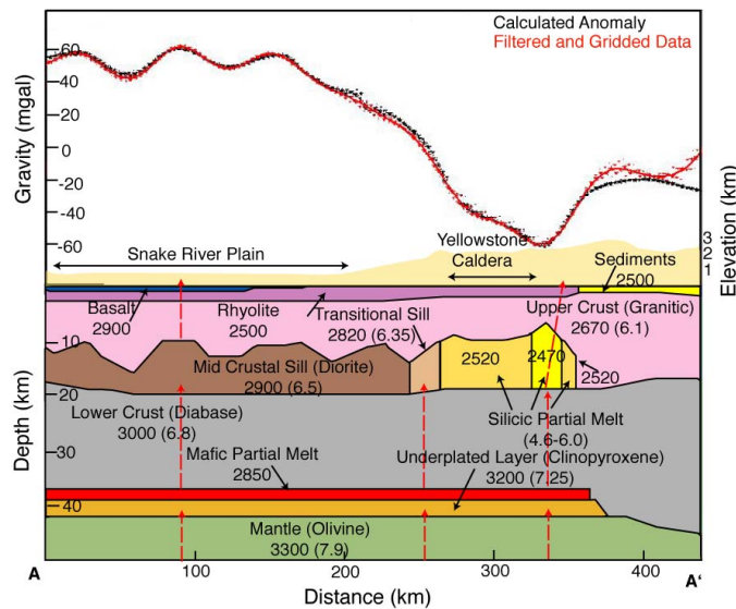
Fig. 12: Cross-section of the YSRP density model reflecting the results of previous studies and the velocity density composition analysis of this study. Numbers in parentheses represent P -wave velocities (km/s). Shading above cross section represents the generalized topography.
