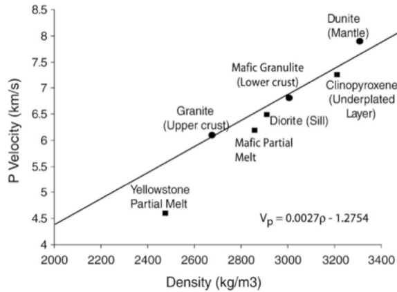
Fig. 9: Velocity-density plot for rocks in the YSRP volcanic field. Circles are rocks with densities inferred from other studies, squares are densities of rocks evaluated in this study. The Yellowstone upper crustal partial melt and mafic melt were not included in the calculation of the linear equation.
