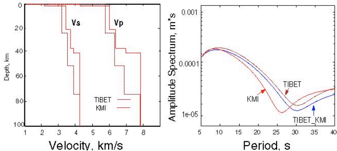
Figure 10. The differences in synthetic amplitude spectra for the path from Tibet to station KMI and a realistic source mechanism. Left: crustal models under the source (TIBET) and receiver (KMI). Right: Synthetic amplitude spectra for three different simulations. TIBET curve is for TIBET model at both event and station locations; KMI curve is for KMI model at both locations; TIBET-KMI curve is for TIBET model near the source and KMI model under the station.
