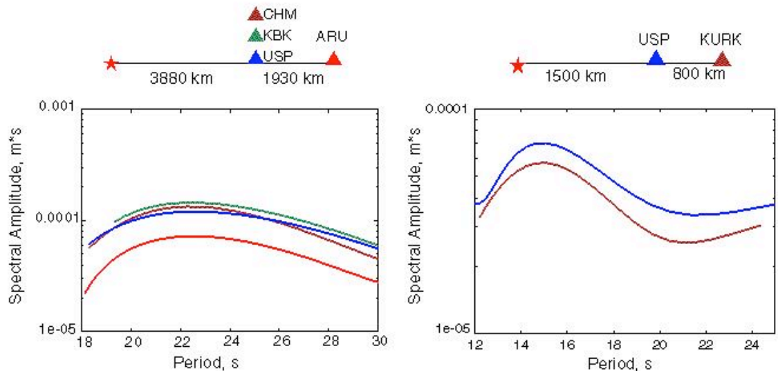
Figure 8. Examples of inter-station measurements by stations of KAZNET and KNET networks. Left: Event near Andaman Islands; Right: Event in Pakistan.
